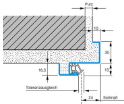
Eckzarge (EZS), Profil 21
