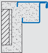
Turnhalleneckzarge
